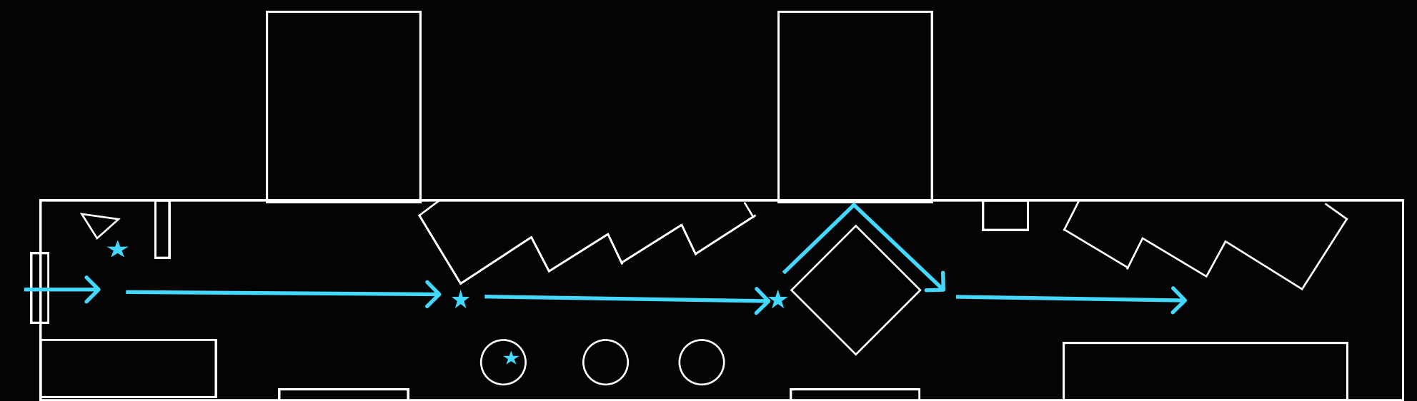
Figure 8. Museum floor plan and dynamic line analysis.
